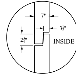
JOINT DETAIL SINGLE OFFSET GASKET PER ASTM C-443 AND C-990
