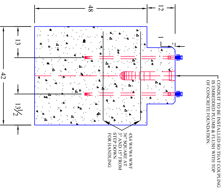
SECTION B-B'
