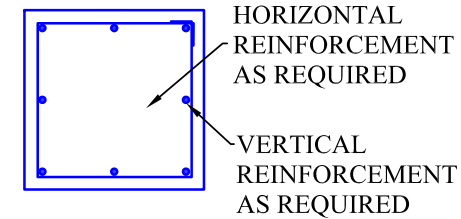
PLAN VIEW REINFORCEMENT
