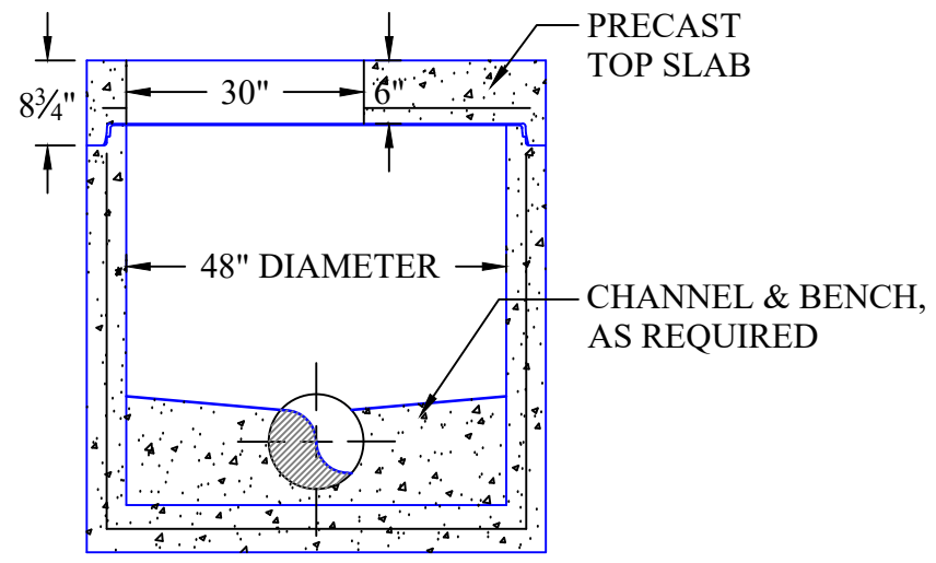
SECTION WITH SLAB TOP
