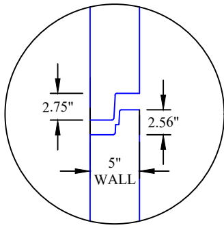
JOINT DETAIL RUBBER GASKET PER ASTM C-443 BUTLY RUBBER GASKET PER ASTM C-990
