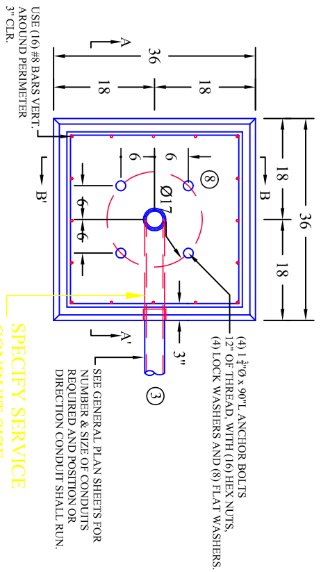
PLAN VIEW
