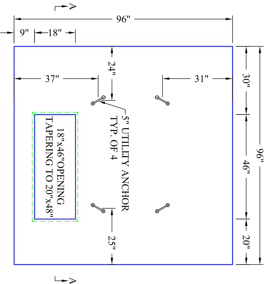
PLAN VIEW
