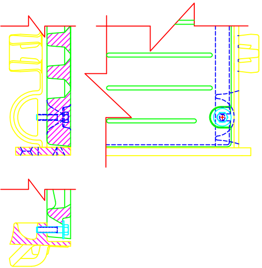
FRAME & GRATE SHOWING DEBRIS CHUTE
