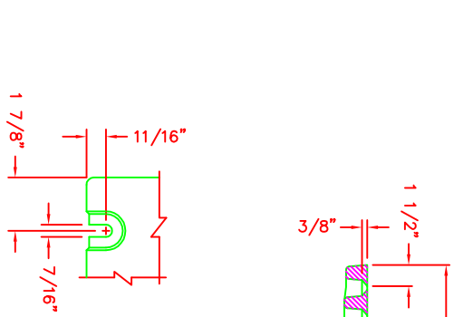
BOLT SLOT DETAIL SCALE 1:4
