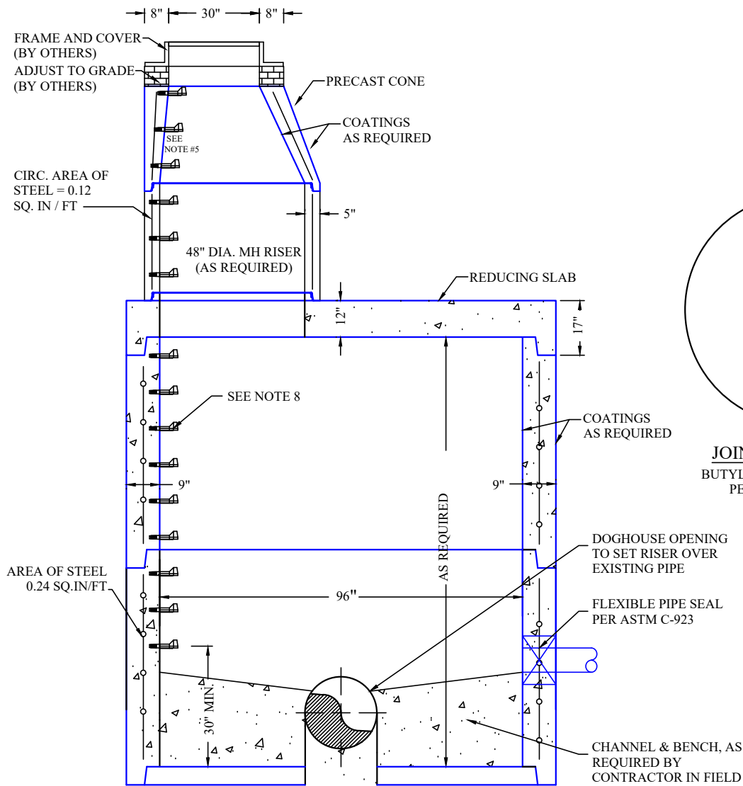
96" DIAMETER MANHOLE WITH REDUCING SLAB
