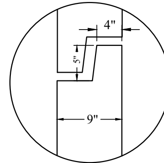
JOINT DETAIL BUTYL RUBBER GASKET PER ASTM C-990
